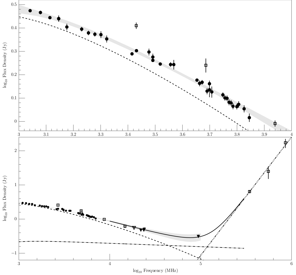
Figure 4.9: Spectrum of the core component of NGC 253 with model. The symbols are as in Figure 4.8. External data are found in Beck et al. (1979) ; Hildebrand et al. (1977) ; Ott et al. (2005) ; Peng et al. (1996) ; Ricci et al. (2006) ; Rieke et al. (1973) ; Takano et al. (2005) ; Weiss et al. (2008) . See §4.4.2 for discussion.
