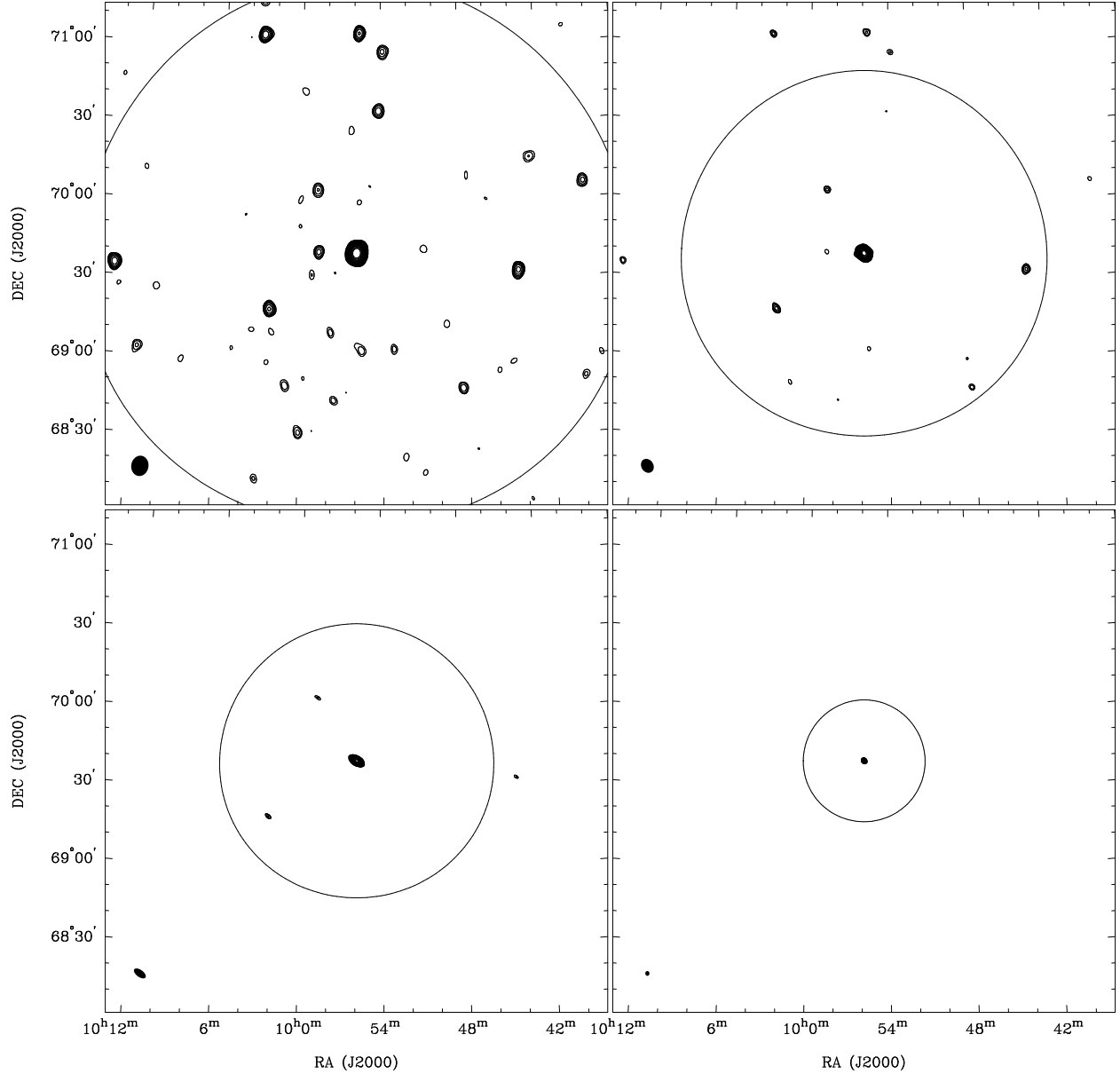
Figure 4.5: ATA maps of M82 at 1.0, 1.5, 2.0, and 4.5 GHz (top left, top right, bottom left, and bottom right panels, respectively). The depicted maps are the reference images at each frequency reimaged onto a common coordinate grid. Circles : half-power points of the ATA beam. Filled ellipses : synthesized beamsizes. Contour levels in all panels are 50 \text{ mJy} \times 2^{n/2} for n = 0, 1, 2, \dots, 13 . The RMS noise levels of the images are 17, 13, 10, and 11 mJy. The number of sources seen decreases as frequency increases due to both the shrinking primary beam of the telescope and the general downward slope of the radio spectra of celestial sources.
