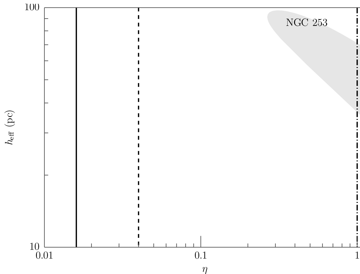
Figure 4.15: Values of \eta and h_{\text{eff}} for which spectral curvature parameters B and C derived from the T+06 model are consistent with observations of NGC 253 to within 2\sigma . The symbols are as in the previous figure. Shaded region: the allowed parameters for p = 2 . The T+06 model with p = 2.3 is excluded to a 99.99% confidence limit.
